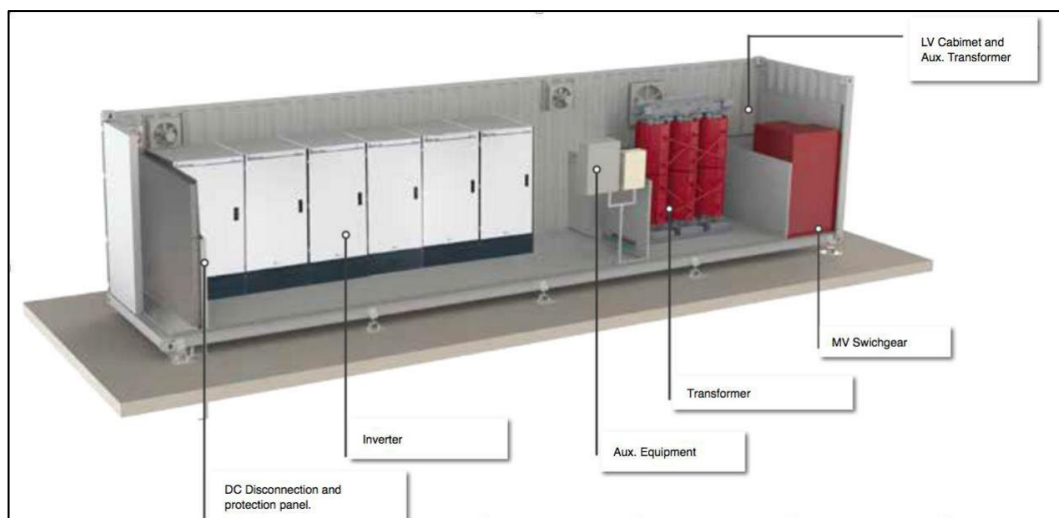
Image 4-4 Typical Integrated Conversion Unit
